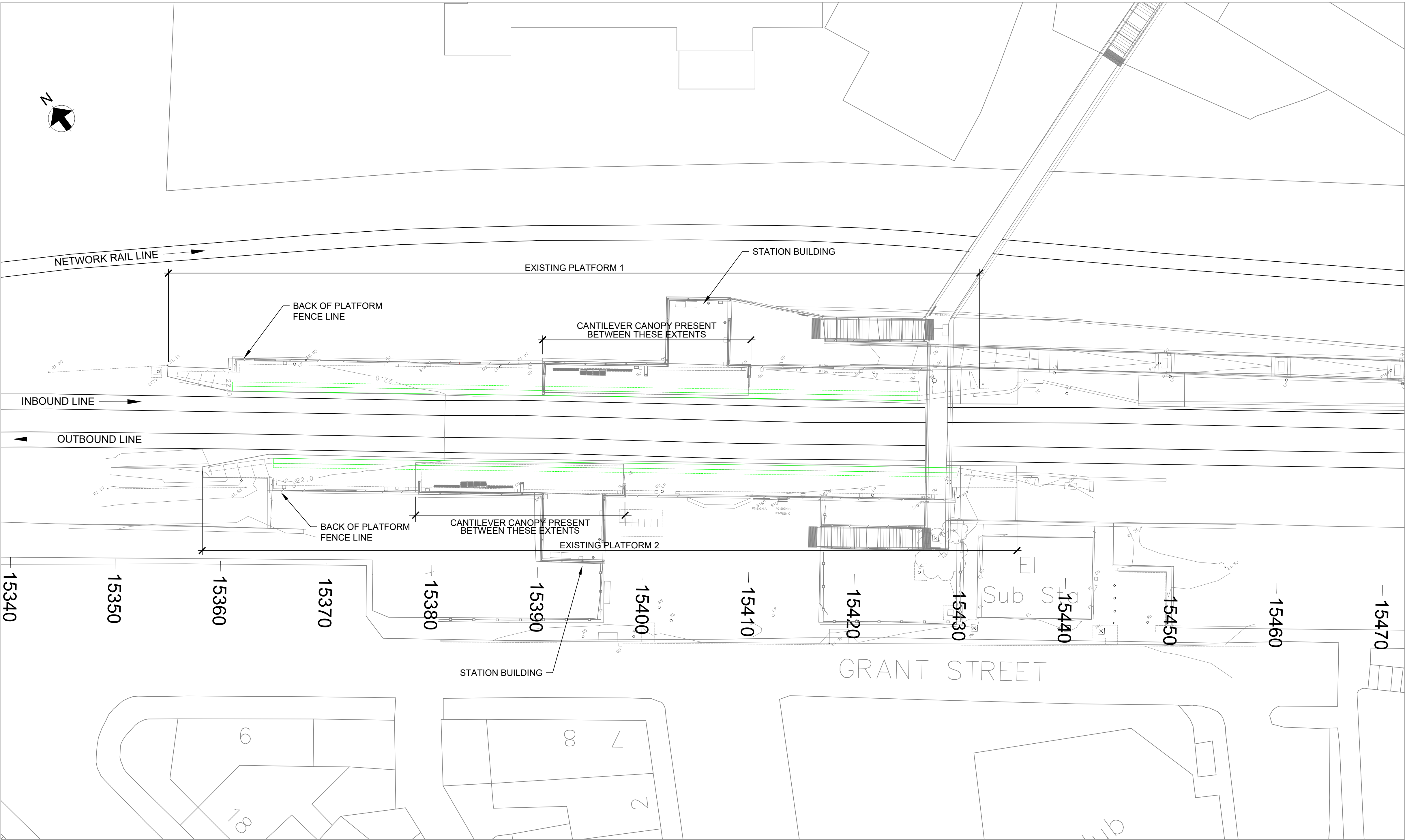
PLAN - 1:200
