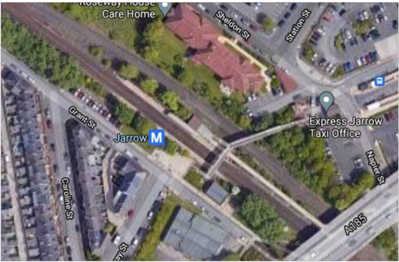
JARROW STATION PLATFORM 1 & 2 - NTS
